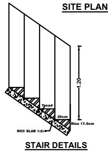
STAIR DETAILS
