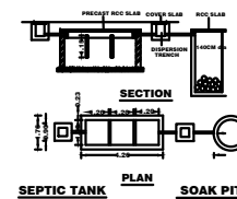
SEPTIC TANK SOAK PIT
