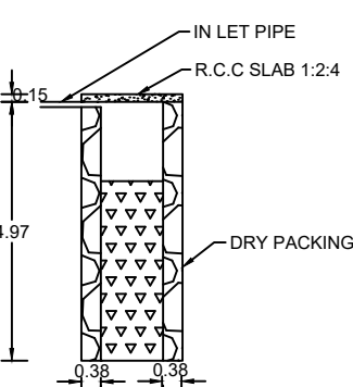
WASTE WATER TANK
