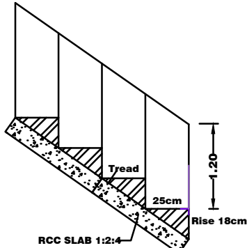
STAIR DETAILS
