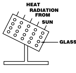
SOLAR SYSTEM
