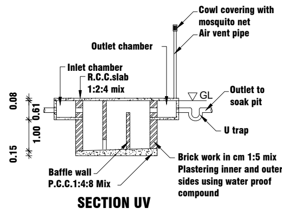
SECTION UV
