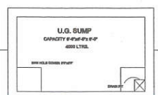
SUMP PLAN
