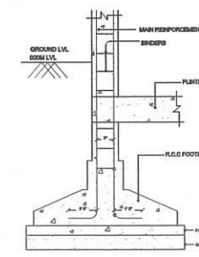
TYPICAL SECTION OF R.C.C COLUMN FOUNDATION
