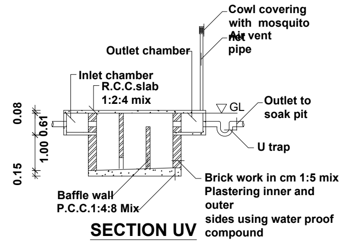
SECTION UV
