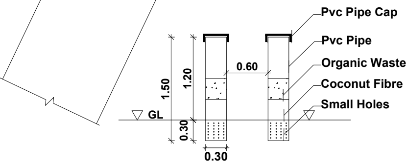
PIPE COMPOST PIT
