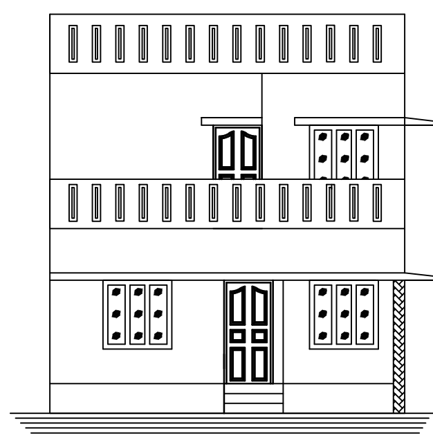
FRONT ELEVATION
