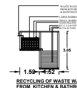
RECYCLING OF WASTE WATER FROM KITCHEN & BATHROOM
