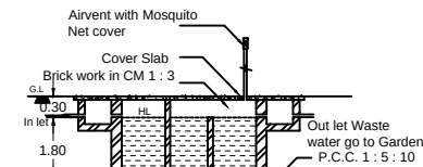
SEPTIC TANK SECTION
