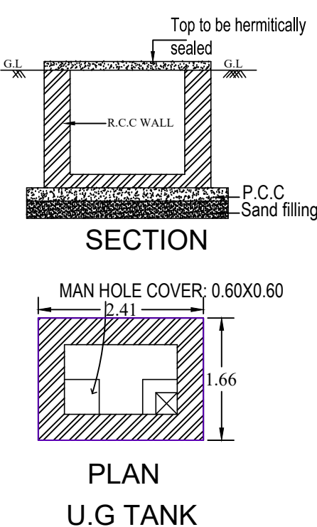
RECYCLING OF WASTE WATER FROM KITCHEN & BATHROOM NOT IN SCALE
