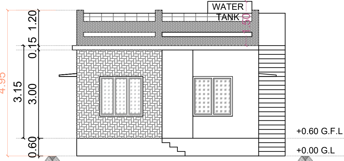
ELEVATION SCALE 1:100
