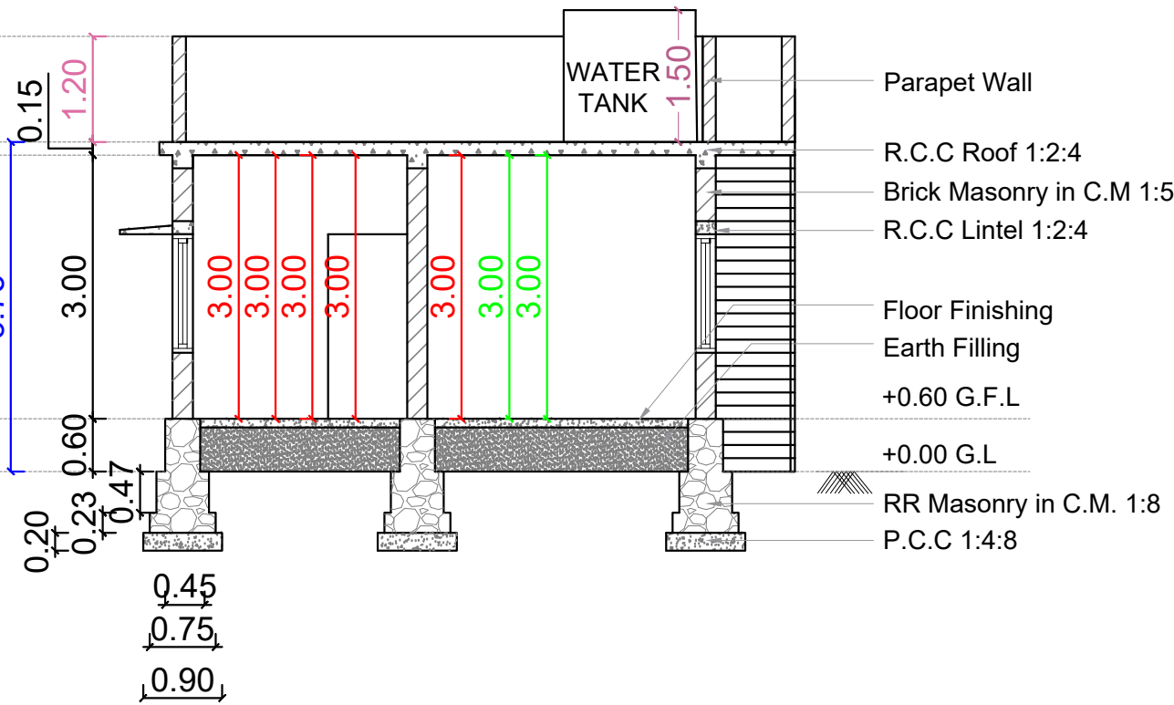
SECTION SCALE 1:100
