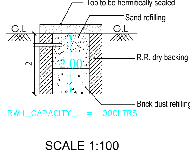
TRAIL PIT SCALE 1:100
