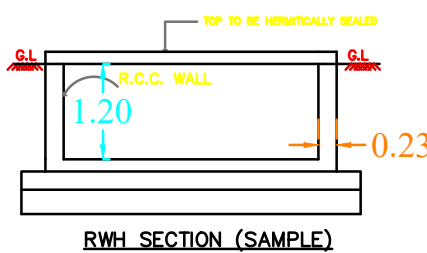
RWH_CAPACITY_L = 2000LTRS
