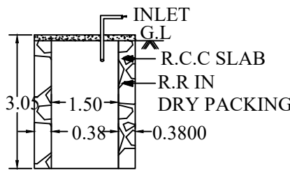
RAIN WATER HARVERSTING
