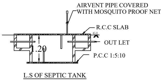
L.S OF SEPTIC TANK
