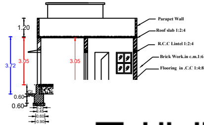
FRONT ELEVATION
