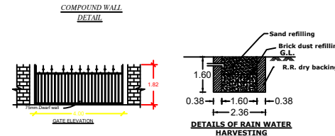
DETAILS OF RAIN WATER HARVESTING
