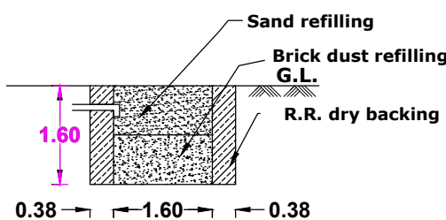
DETAILS OF RAIN WATER HARVESTING Dwg:1A
