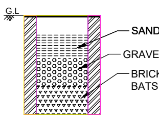
RAIN WATER PIT
