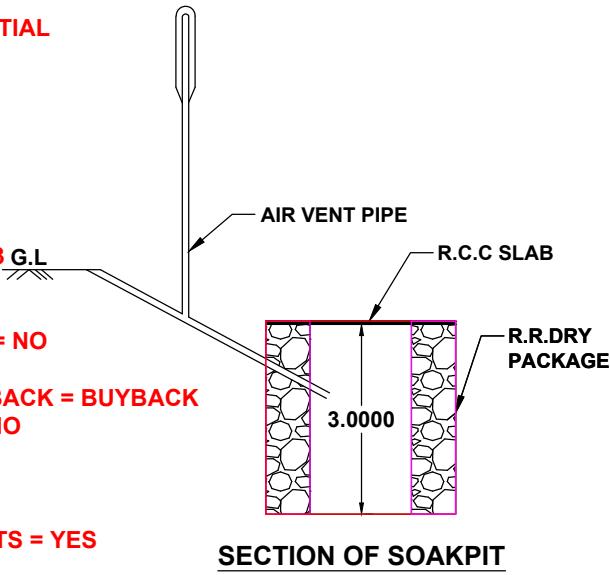
SECTION OF SOAKPIT
