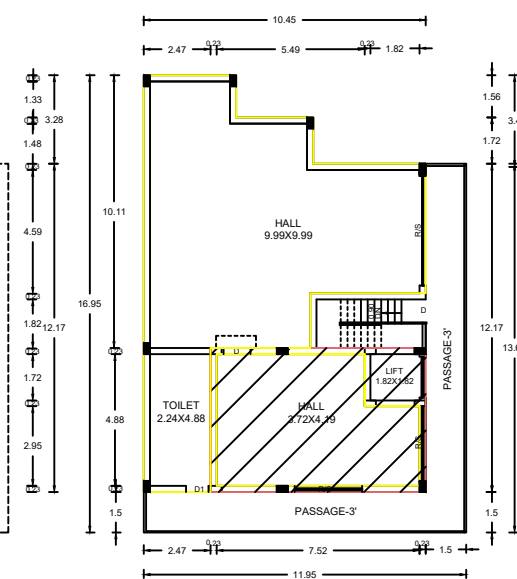
EXISTING APPROVAL NO:51/2024 AND PROPOSED FIRST FLOOR PLAN
