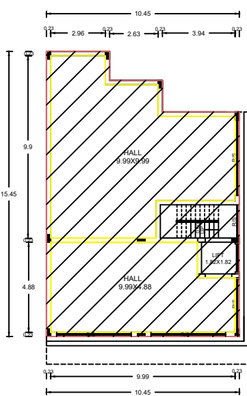
EXISTING APPROVAL NO:51/2024 GROUND FLOOR PLAN
