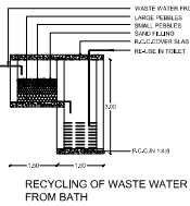
RECYCLING OF WASTE WATER FROM BATH
