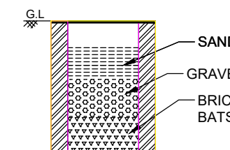
RAIN WATER PIT
