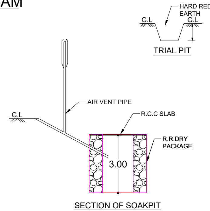
SECTION OF SOAKPIT
