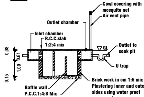
SECTION UV
