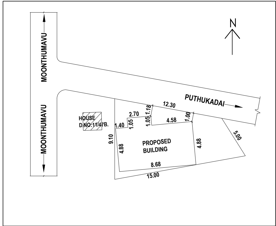
KEY PLAN
