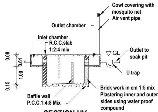
SECTION UV
