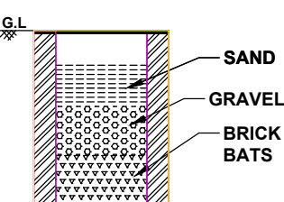
RAIN WATER PIT
