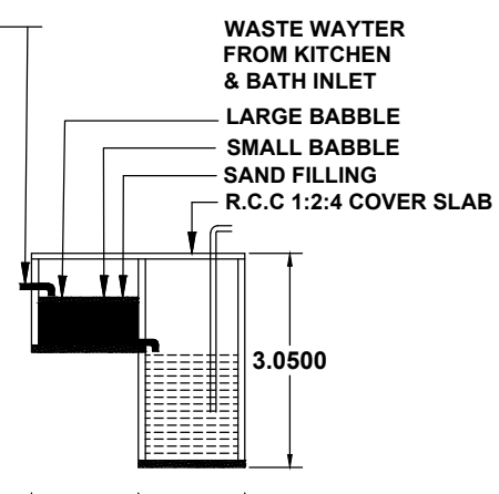
RECYCLING OF WASTE WATER TANK
