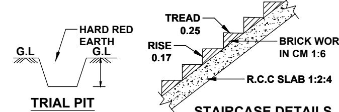
STAIRCASE DETAILS
