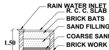
RAIN WATER HARVESTING PIT
