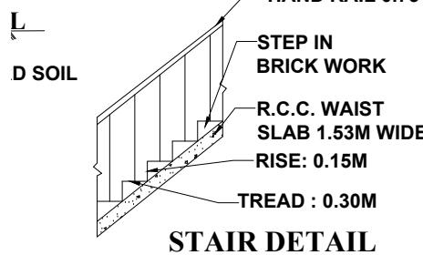
STAIR DETAIL
