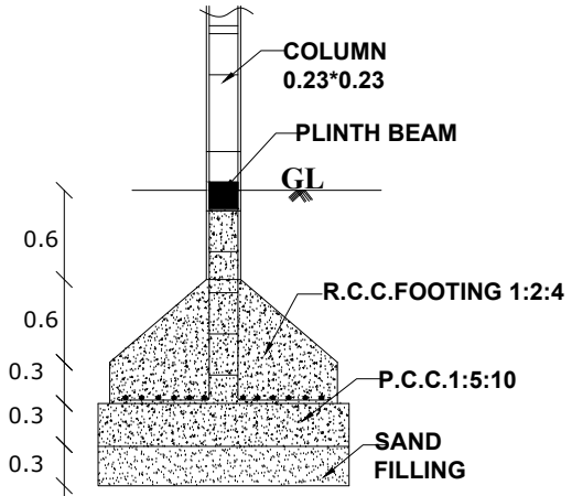
COLUMN DETAILS DETAIL "A"
