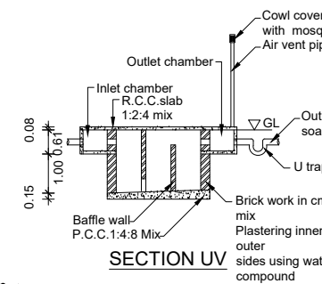
SECTION UV
