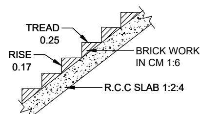
STAIRCASE DETAILS
