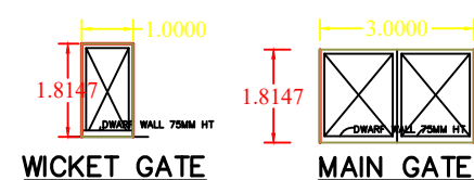
WICKET GATE
