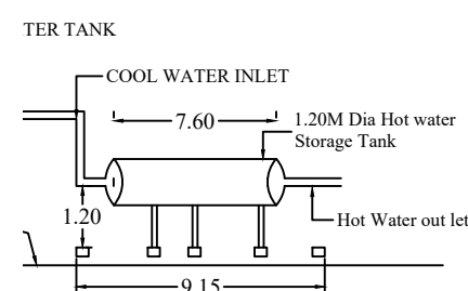
WATER HEATING SYSTEM ( S.W.H.S.DETAILS)
