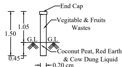
PIPE COMPOSTER
