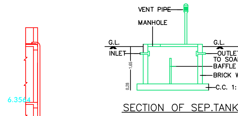
SECTION OF SEP.TANK
