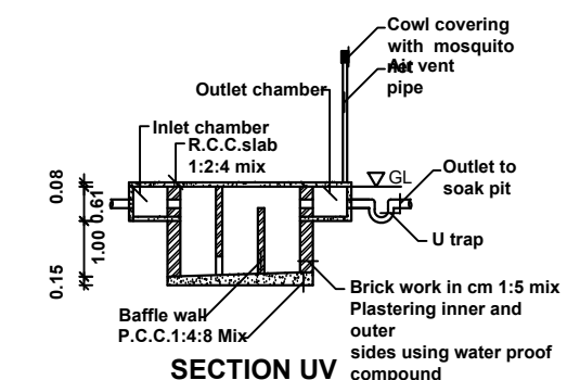
SECTION UV
