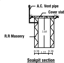
Soakpit section
