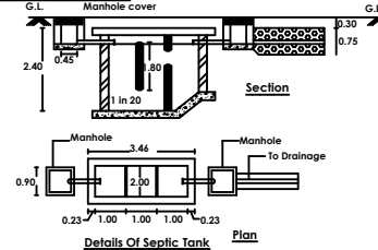
Details Of Septic Tank
