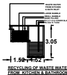
RECYCLING OF WASTE WATER FROM KITCHEN & BATHROOM
