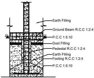
DETAILS OF R.C.C COLUMN
