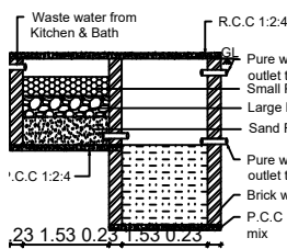
WASTE WATER RECYCLING PIT
