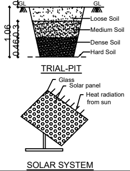
SOLAR SYSTEM
