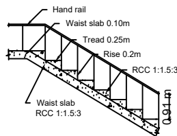
STAIR CASE DETAILS
