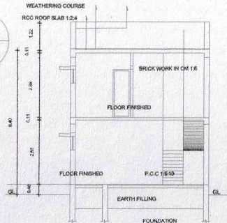
SECTION "A-B"
