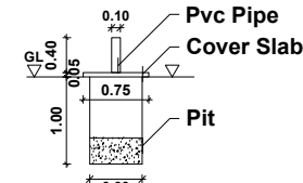
SOLID WASTE COMPOST PIT
