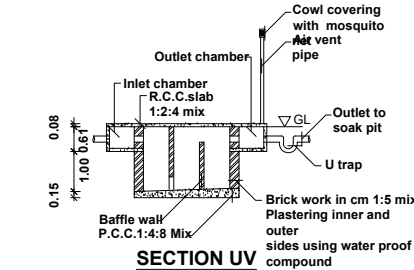
SECTION UV
