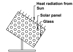
SOLAR SYSTEM
