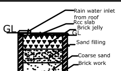
RAIN WATER HARVESTING PIT
