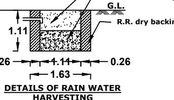
DETAILS OF RAIN WATER HARVESTING
