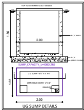
U/S SUMP DETAILS
