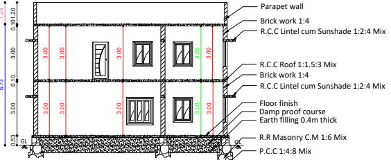
CROSS SECTION
