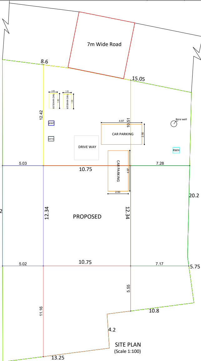
RAIN WATER HARVESTING PIT RWHP CAPACITY: 1,50,000 LTR
