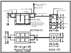
SEPTIC TANK & SOAK PIT
