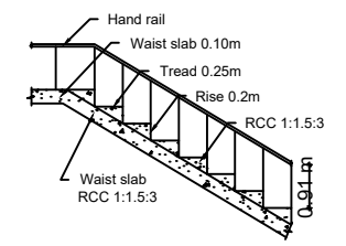
STAIR CASE DETAILS
