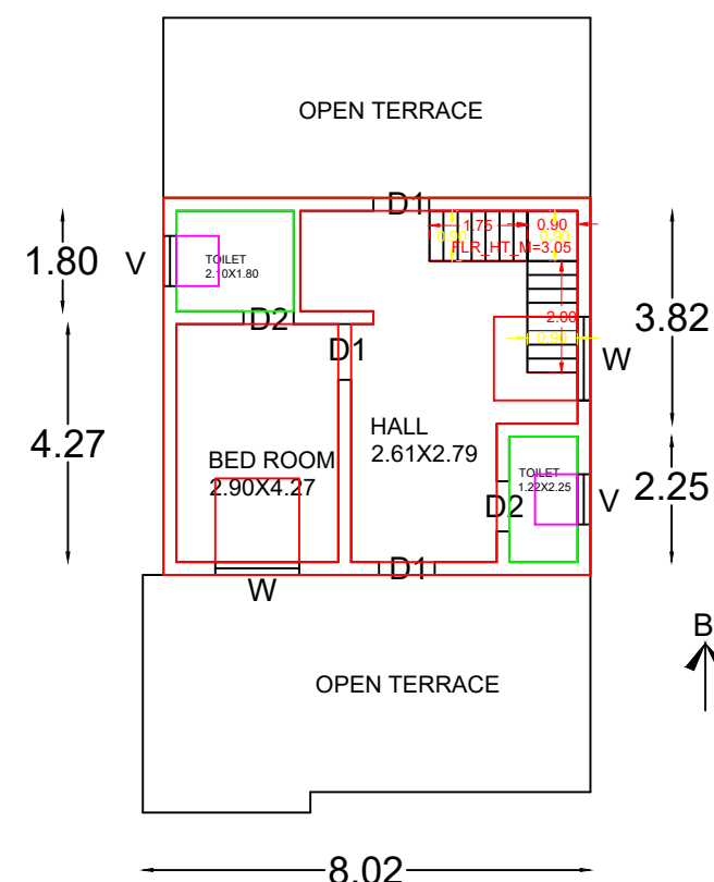
FF PLAN
