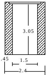
P L A N RAIN WATER HARVESTING ARRANGEMENT DRAWING TYPE 0.45
