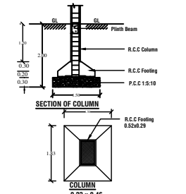
SECTION OF COLUMN
