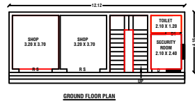
GROUND FLOOR PLAN SCALE 1:100 ALL DIMENSIONS ARE IN METRE
