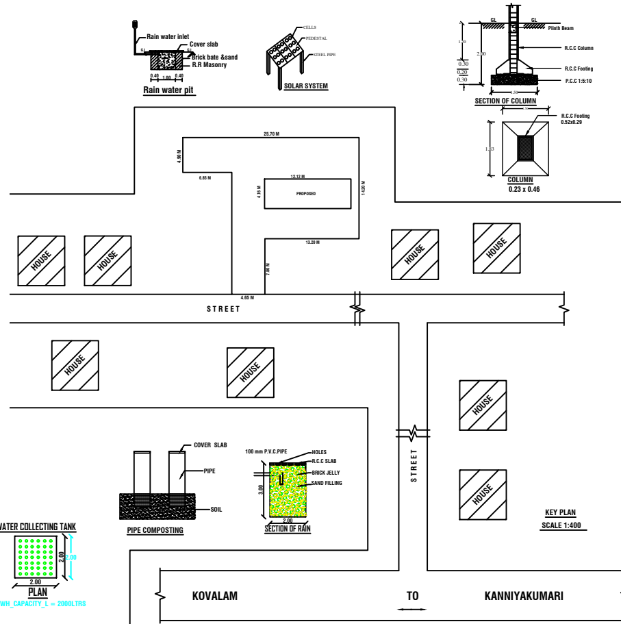
MAIN SITE PLAN
