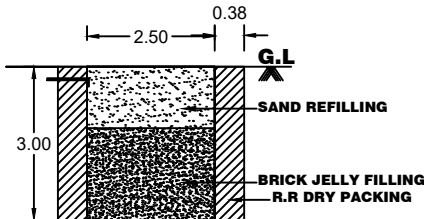
RAINWATER HARVESTING
