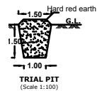
TRIAL PIT (Scale 1:100)
