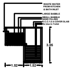
RECYCLING OF WASTE WATER FROM KITCHEN & BATHROOM
