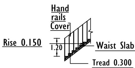
STAIRCASE DETAILS
