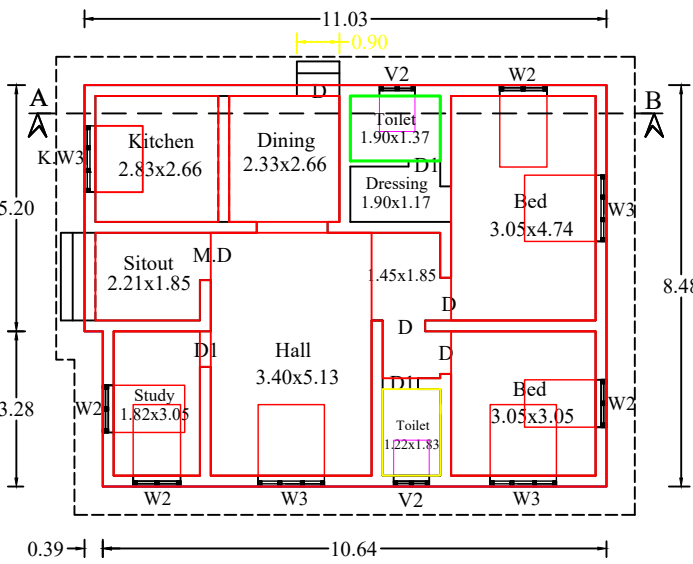
STILT FLOOR PLAN
