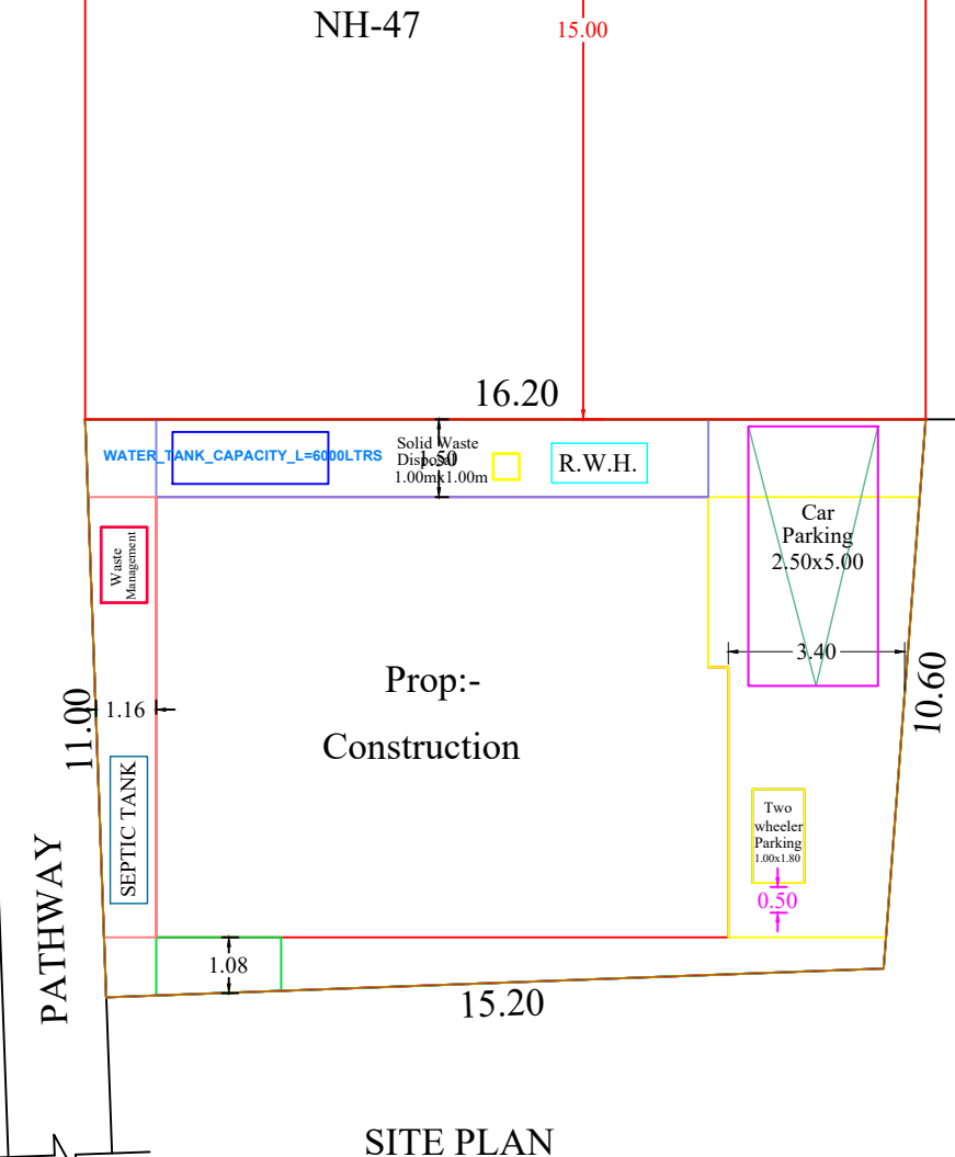
SITE PLAN
