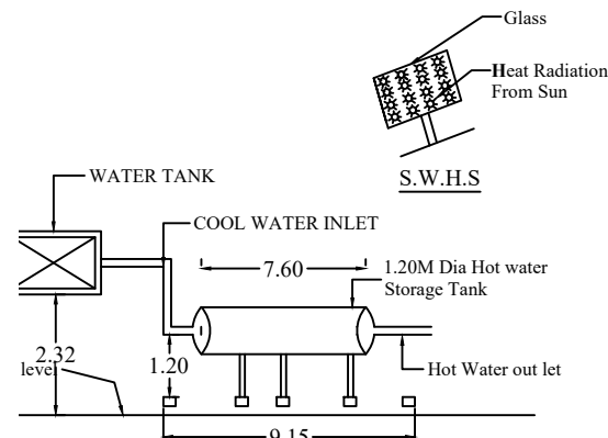
SOLAR WATER HEATING SYSTEM (S.W.H.S.DETAILS)
