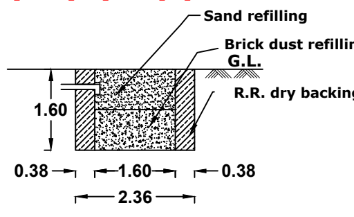
DETAILS OF RAIN WATER
