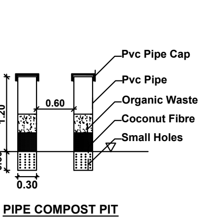
PIPE COMPOST PIT
