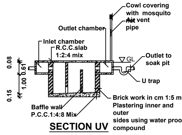
SECTION UV
