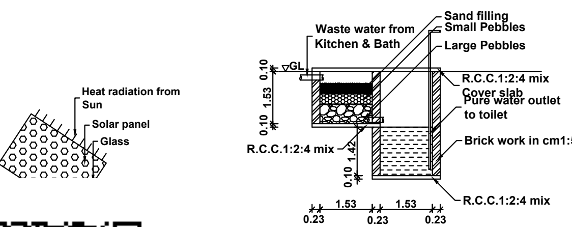
WASTE WATER RECYCLING SYSTEM
