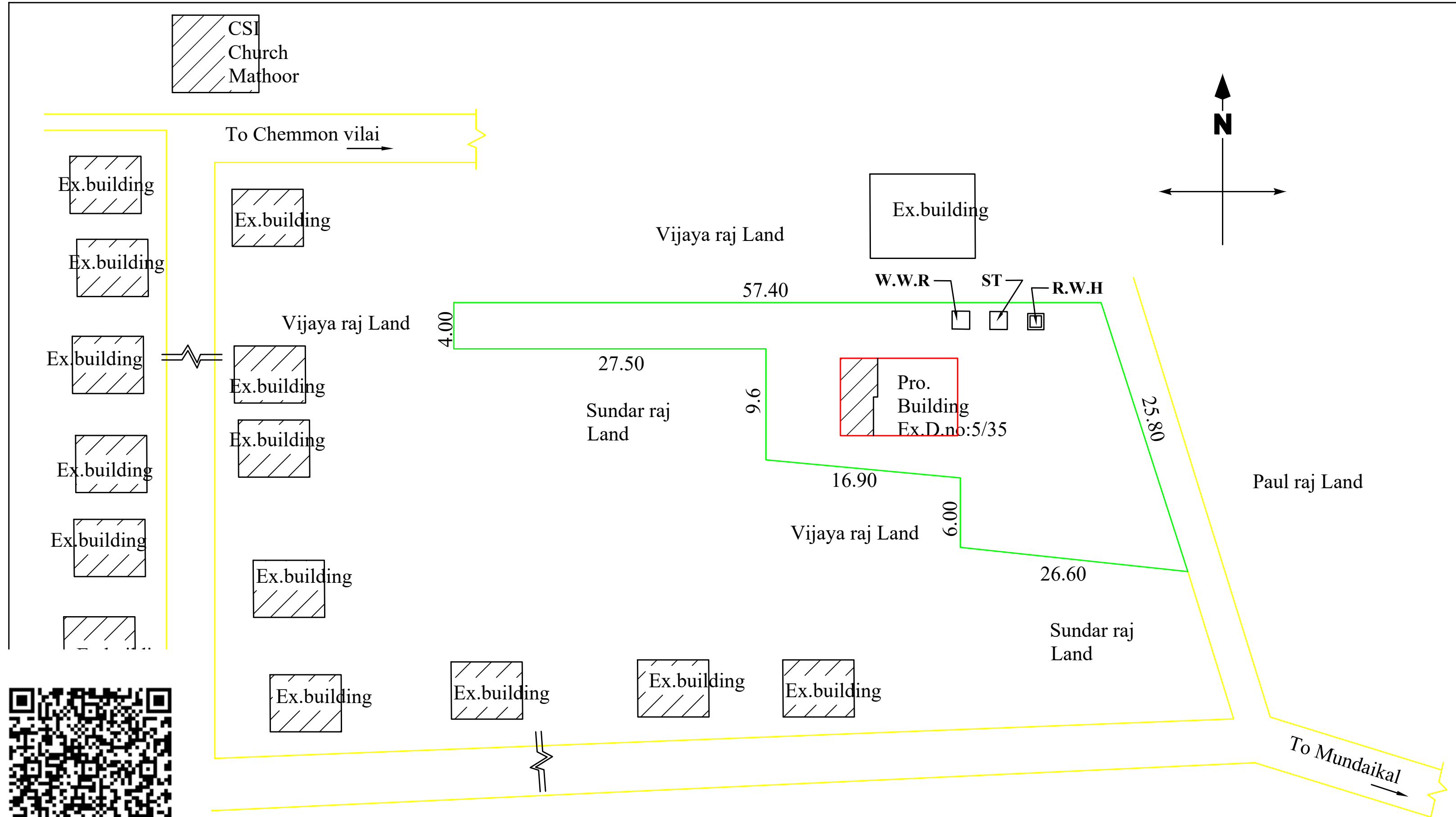
KEY PLAN (SCALE 1:400)
