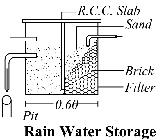
Rain Water Storage
