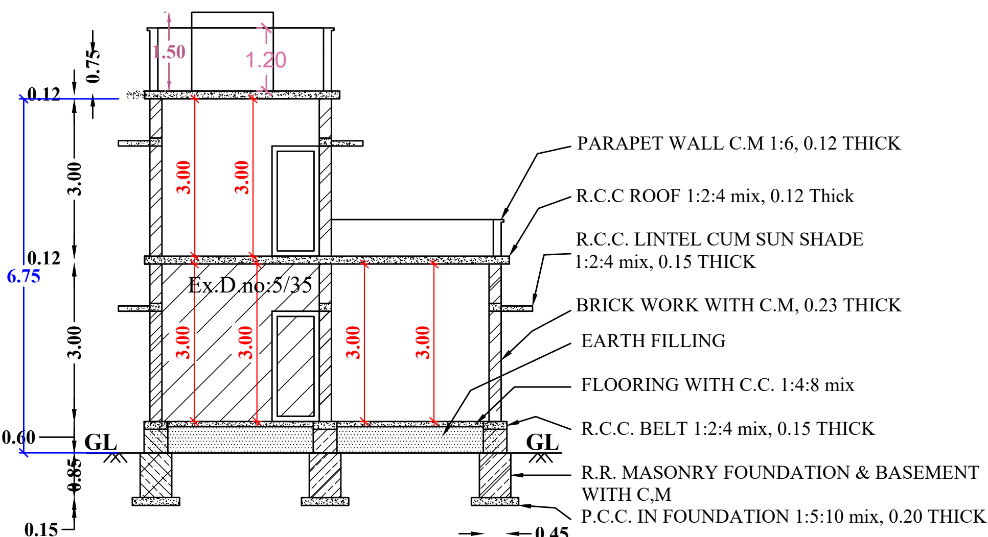
SECTION - AA
