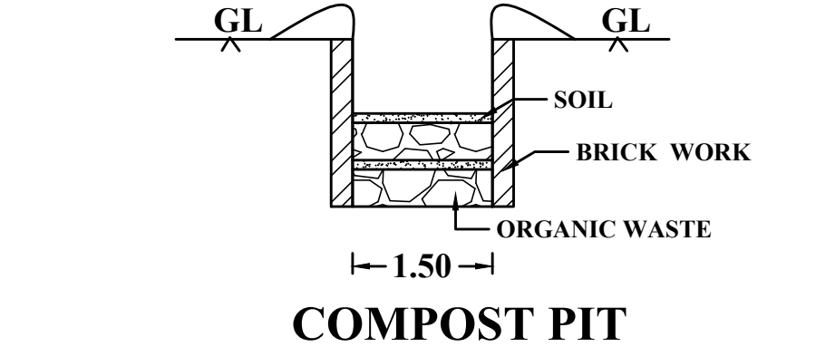
COMPOST PIT
