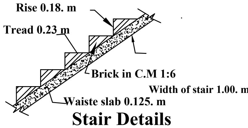
Stair Details
