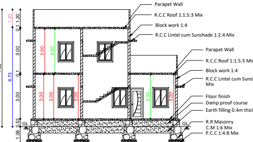
SECTION AB
