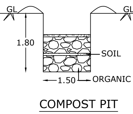
COMPOST PIT
