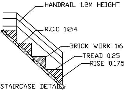
STAIRCASE DETAIL
