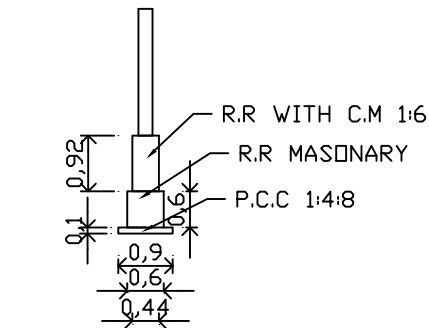
FOUNDATION
