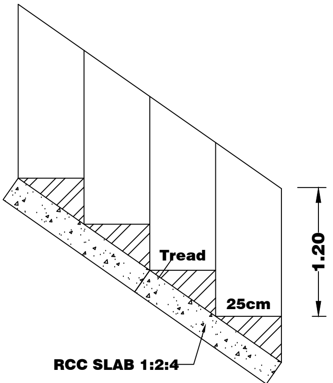
STAIR DETAILS
