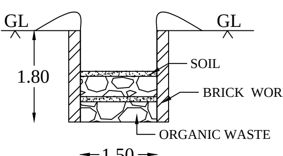
COMPOST PIT
