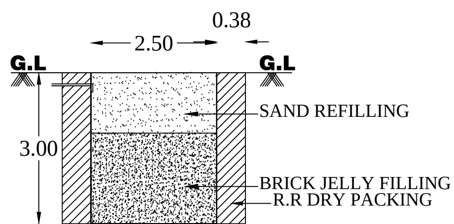
RAINWATER HARVESTING
