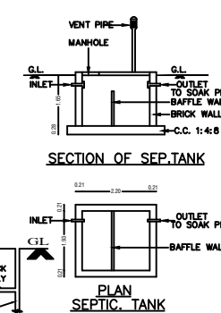
PLAN SEPTIC. TANK
